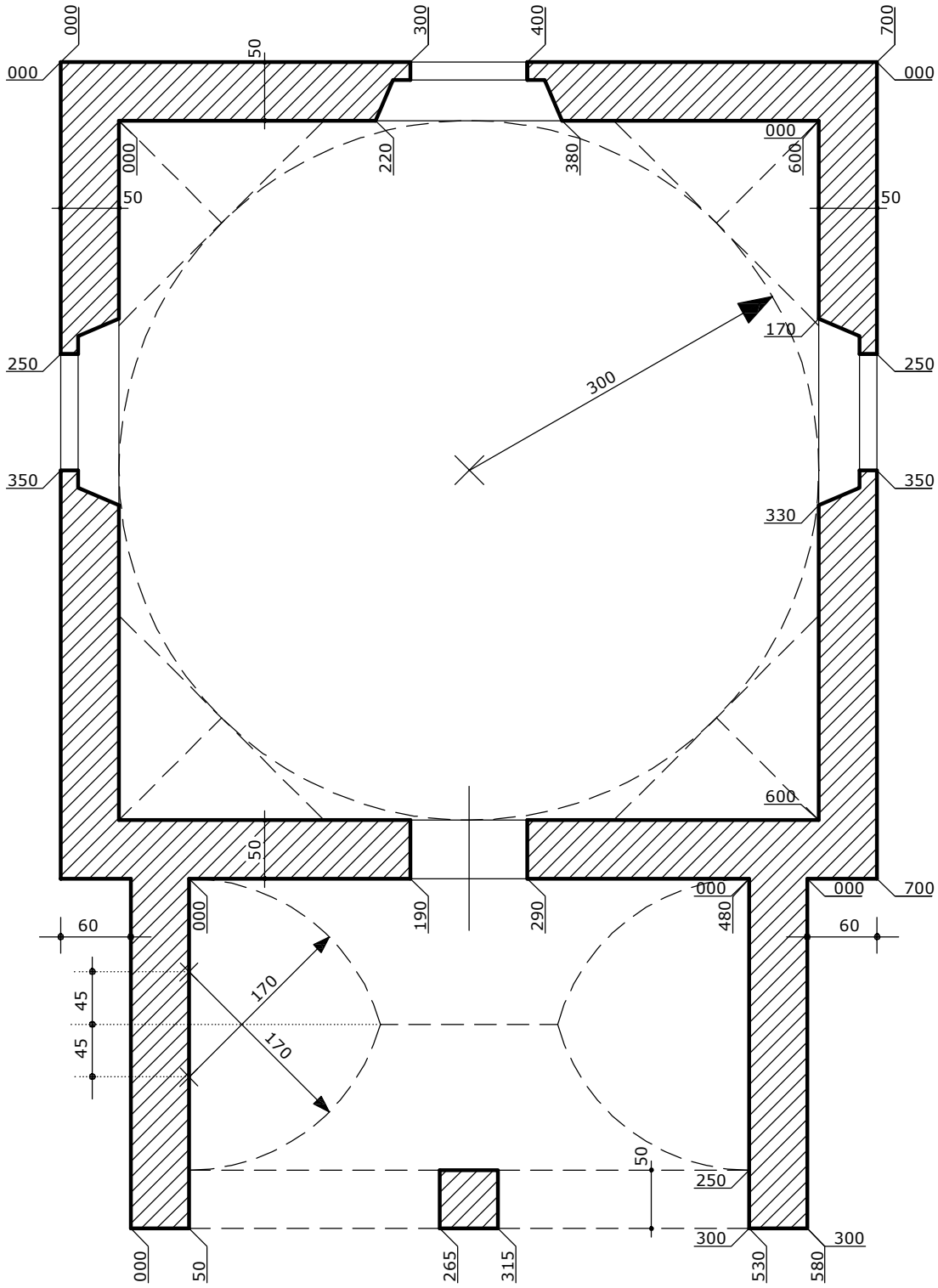
MAZGAL DETAYI
