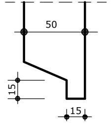
MAZGAL DETAYI
