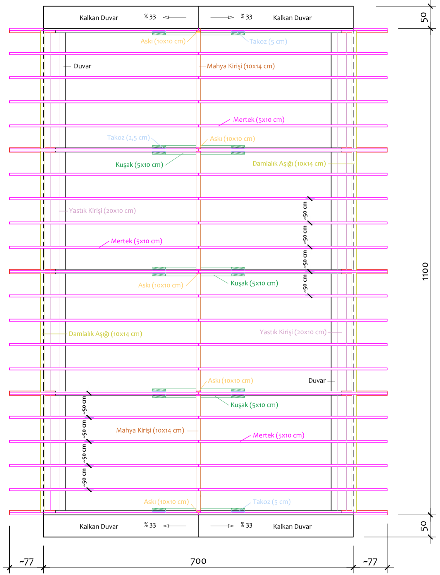
BİR ASKILI AHŞAP ASMA ÇATI PLANI
